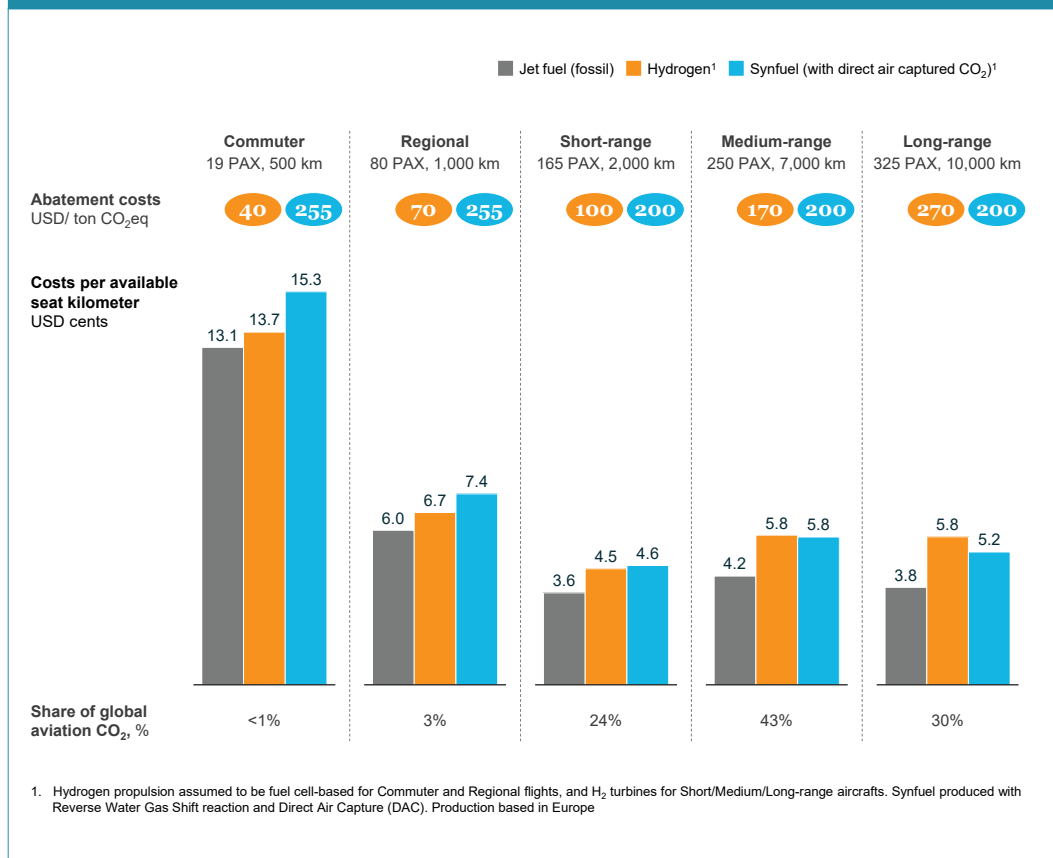
Exhibit 26: Total cost of ownership of aviation fuels for different use cases in 2040
