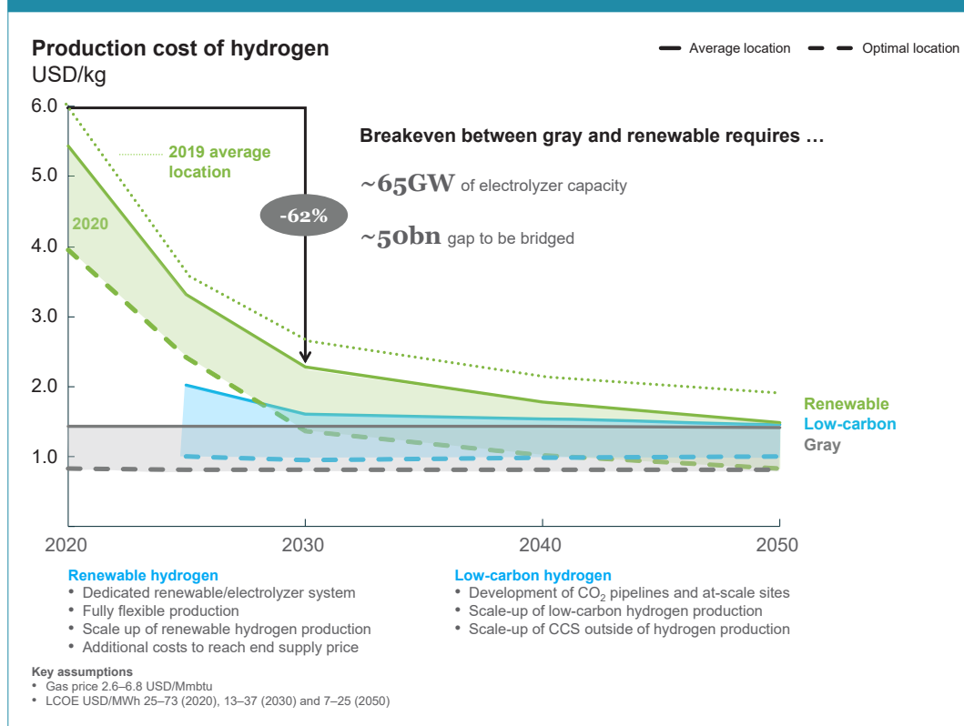
Exhibit 6: Hydrogen production costs by production pathway
