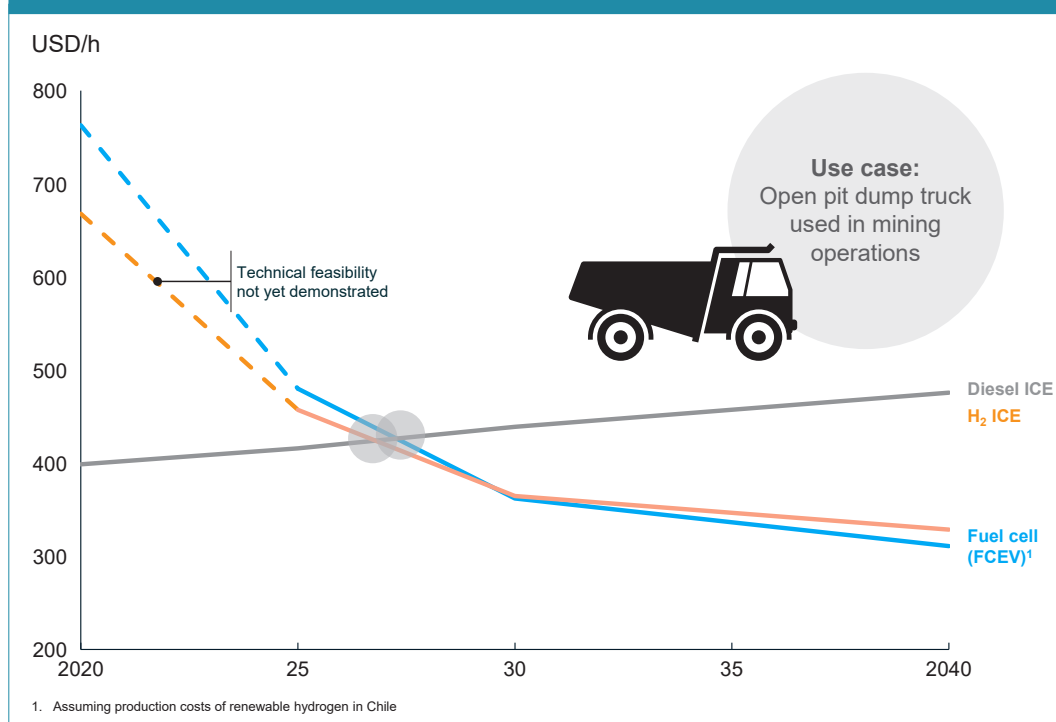
Exhibit 21: Total cost of ownership of a 300 ton open-pit dump truck
